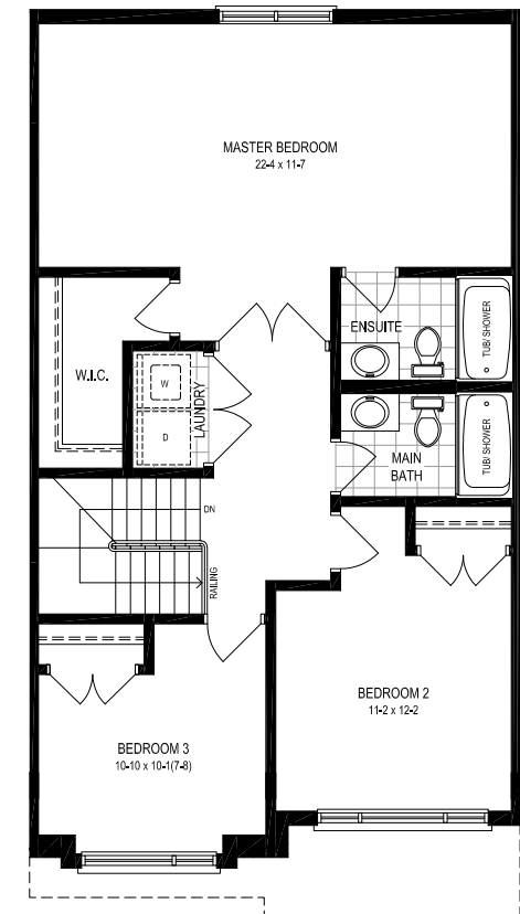
S1 - Second Floor
